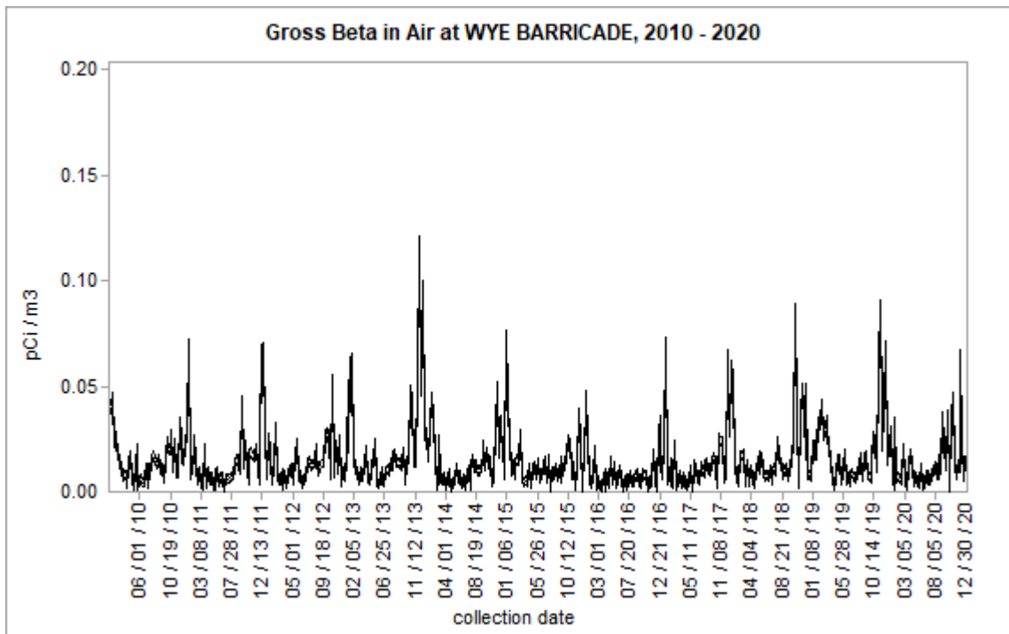
Figure 3.1.17 – Gross Beta in Air at Wye Barricade 2010 - 2020
