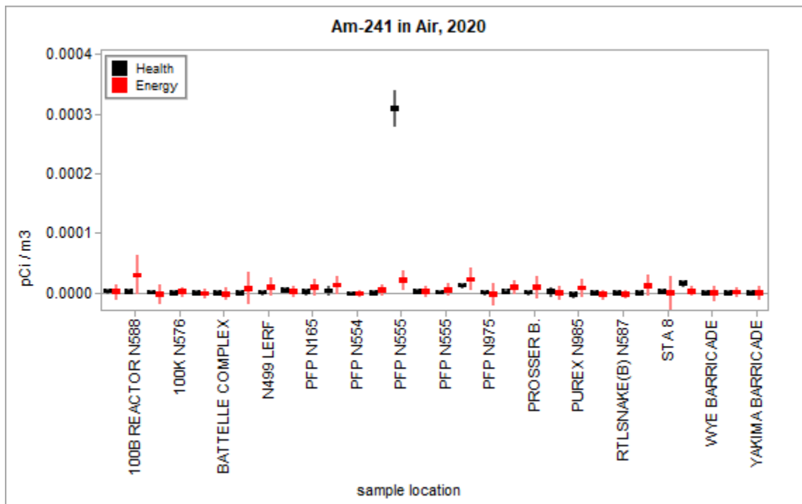
Figure 3.1.9 – Health and Energy Am-241 Concentrations in Air, All Data
