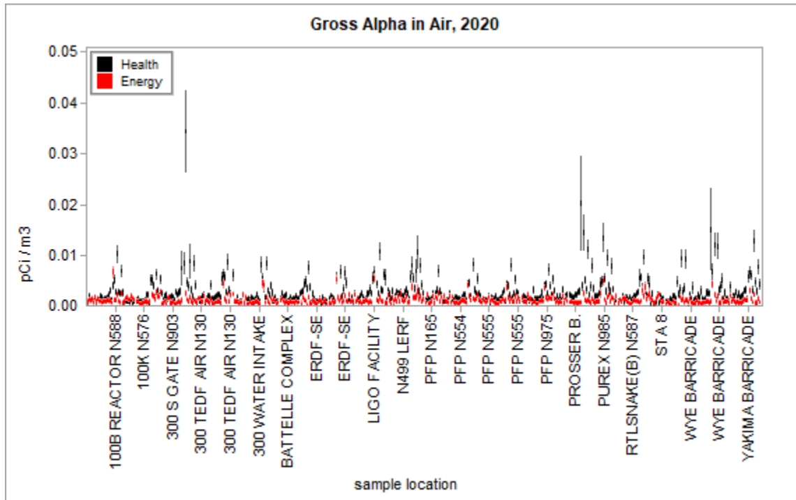
Figure 3.1.2 – Health and Energy Gross Alpha Concentrations in Air
