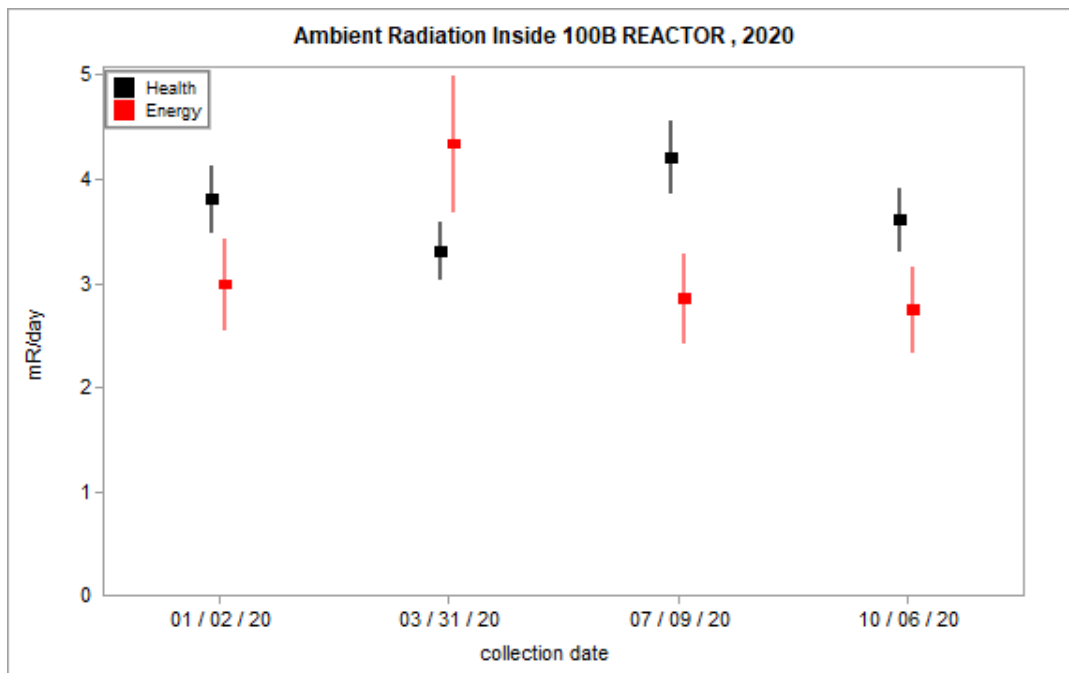
Figure 3.3.3 – Health and Energy Quarterly Ambient Radiation at 100B Reactor
