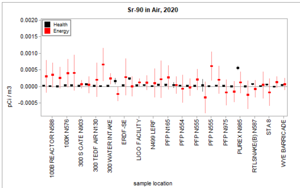
Figure 3.1.15 – Health and Energy Sr-90 Concentrations in Air
