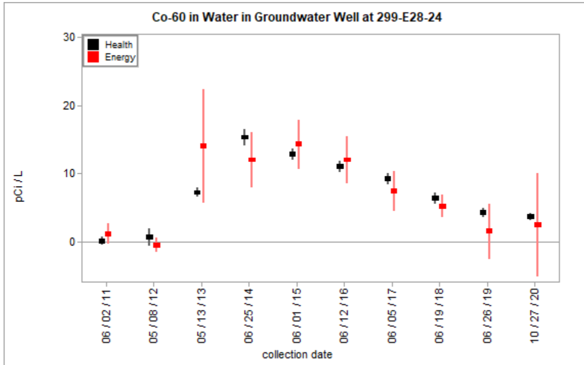
Figure 3.2.4 – Health and Energy Co-60 Concentrations in Water at Groundwater Well 299-E28-24
