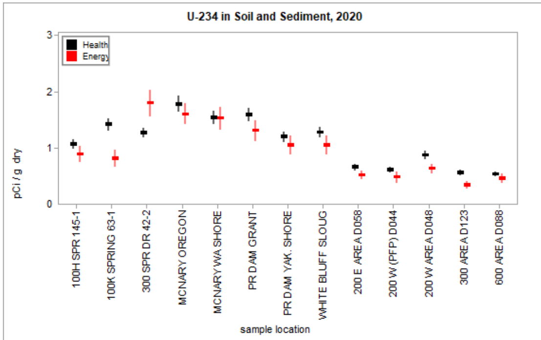
Figure 3.4.8 – Health and Energy U-234 Concentrations in Soil and Sediment
