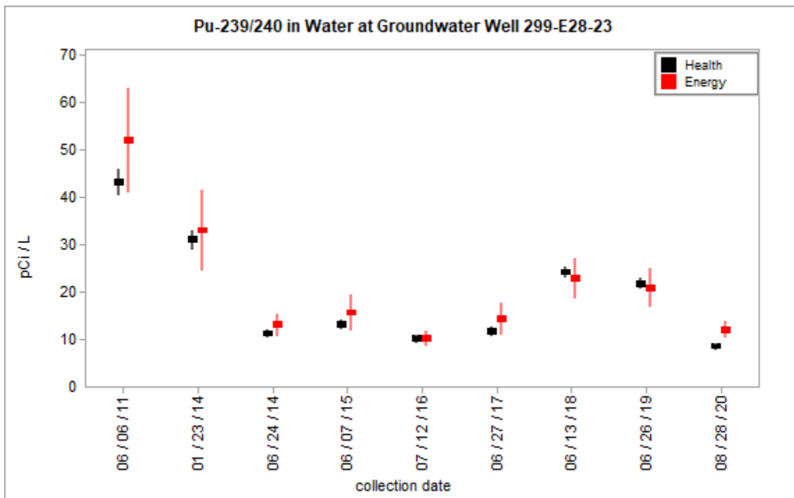
Figure 3.2.12 – Health and Energy Pu-239/240 Concentrations in Water at Groundwater Well 299-E28-23
