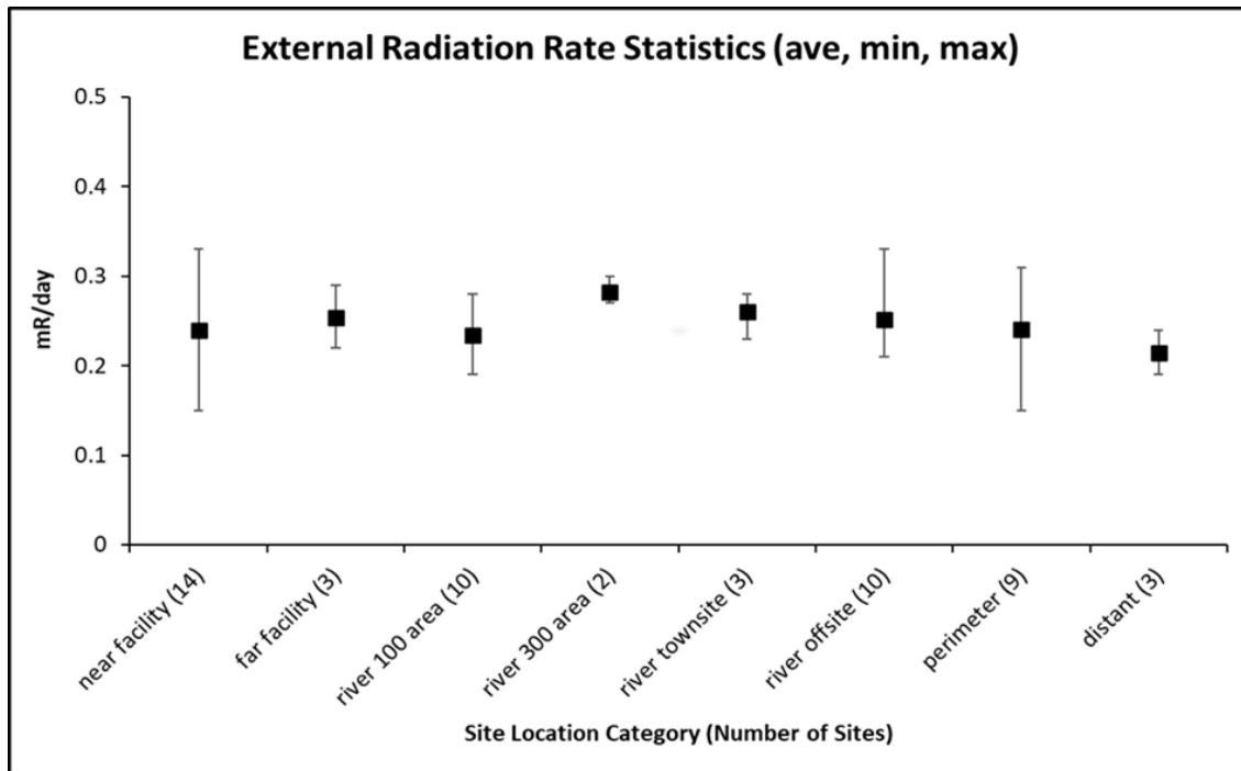
Figure 3.3.4 – Average, Minimum, and Maximum External Radiation Rates by Location Category (data from 2019 Report)
