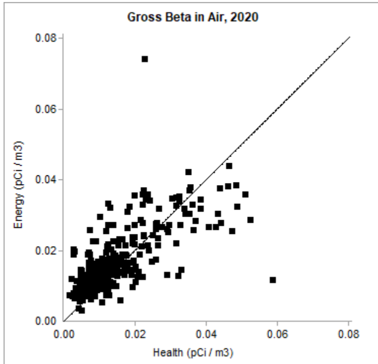
Figure 3.1.6 – Health and Energy Scatter Plot for Gross Beta Concentrations in Air
