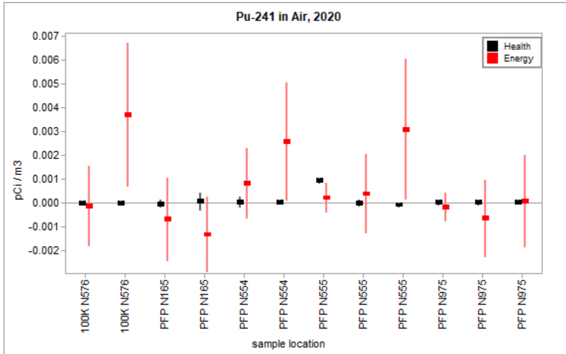
Figure 3.1.14 – Health and Energy Pu-241 Concentrations in Air
