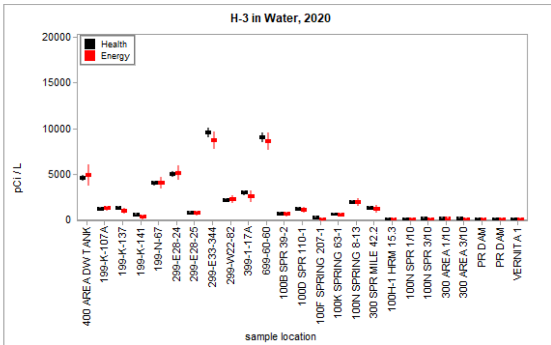
Figure 3.2.8 – Health and Energy H-3 Concentrations in Water, Mid-Range Data
