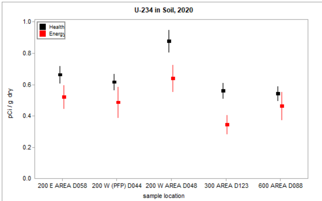
Figure 3.4.9 – Health and Energy U-234 Concentrations in Soil Only
