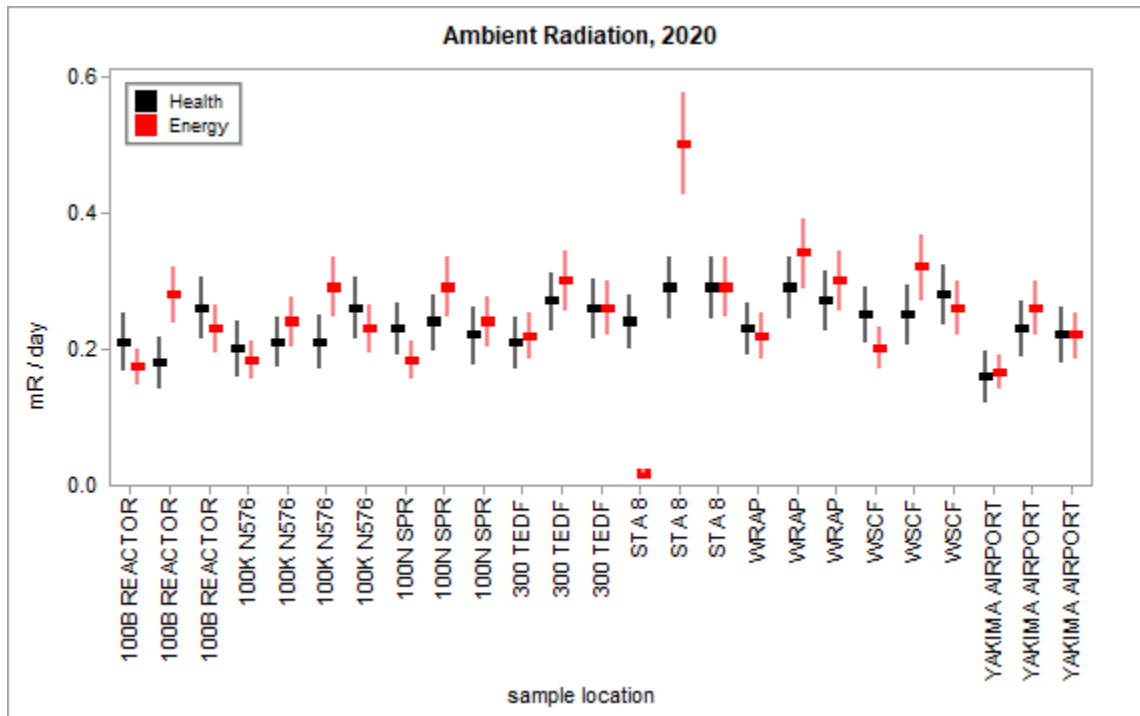
Figure 3.3.2 – Health and Energy Quarterly Ambient Radiation
