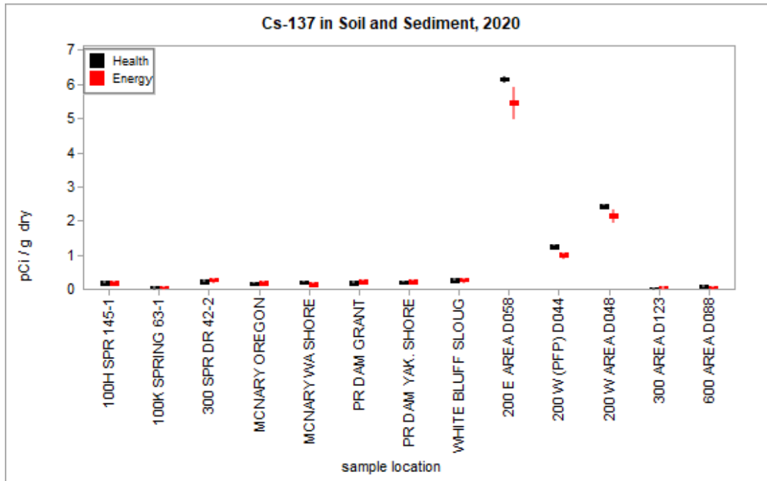
Figure 3.4.3 – Health and Energy Cs-137 Concentrations in Soil and Sediment, Low-Range Data
