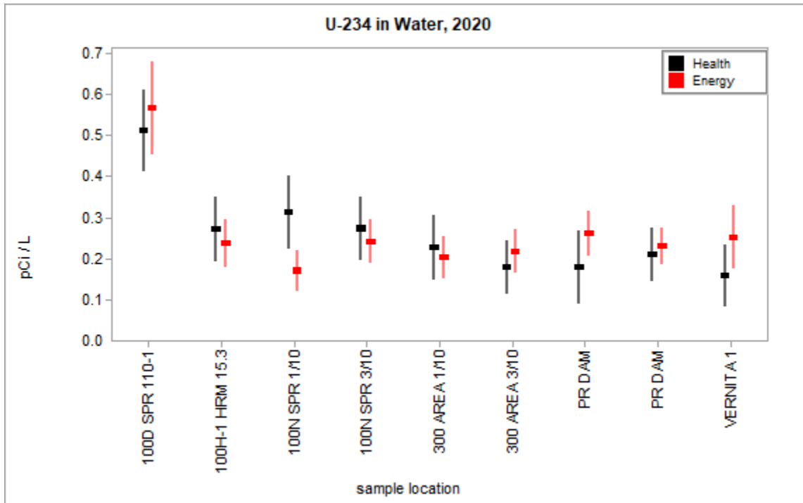
Figure 3.2.17 – Health and Energy U-234 Concentrations in Water, Low-Range Data
