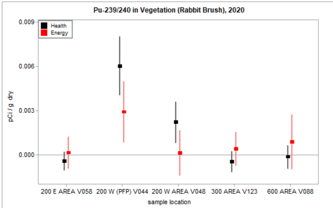
Figure 3.5.1 – Health and Energy Pu-239/240 Concentrations in Vegetation
