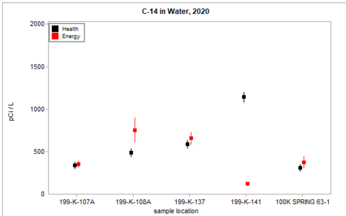
Figure 3.2.3 – Health and Energy C-14 Concentrations in Water, Low-Range Data
