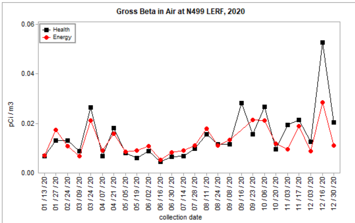
Figure 3.1.5 – Health and Energy Gross Beta Concentrations in Air at Liquid Effluent Retention Facility (LERF)
