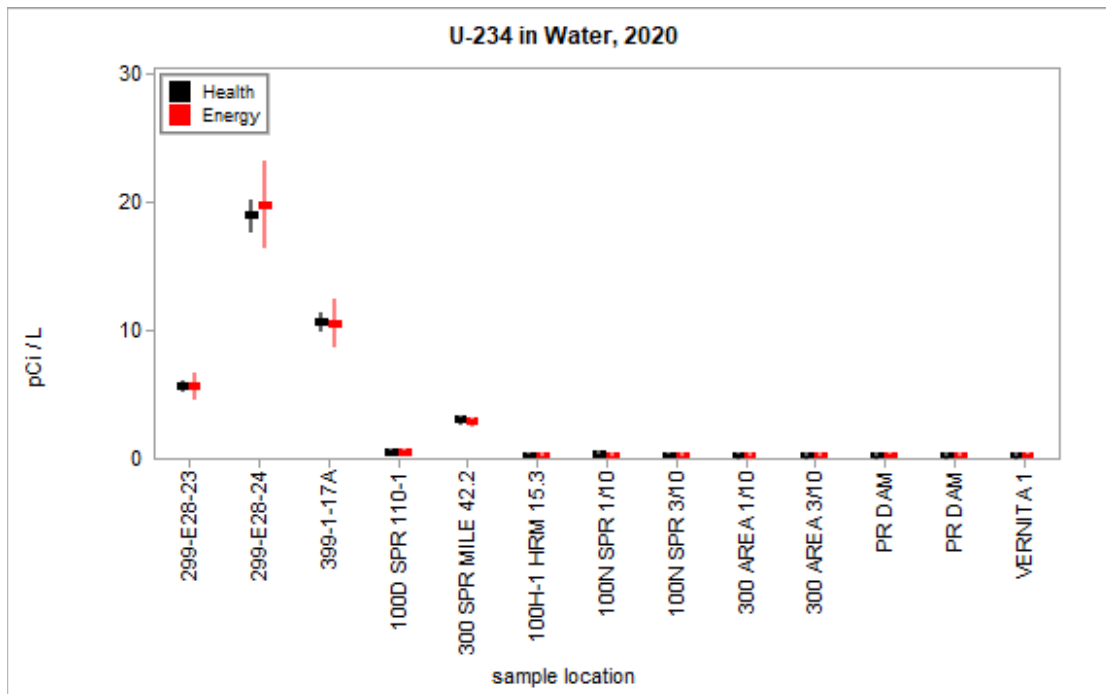
Figure 3.2.16 – Health and Energy U-234 Concentrations in Water, Mid-Range Data
