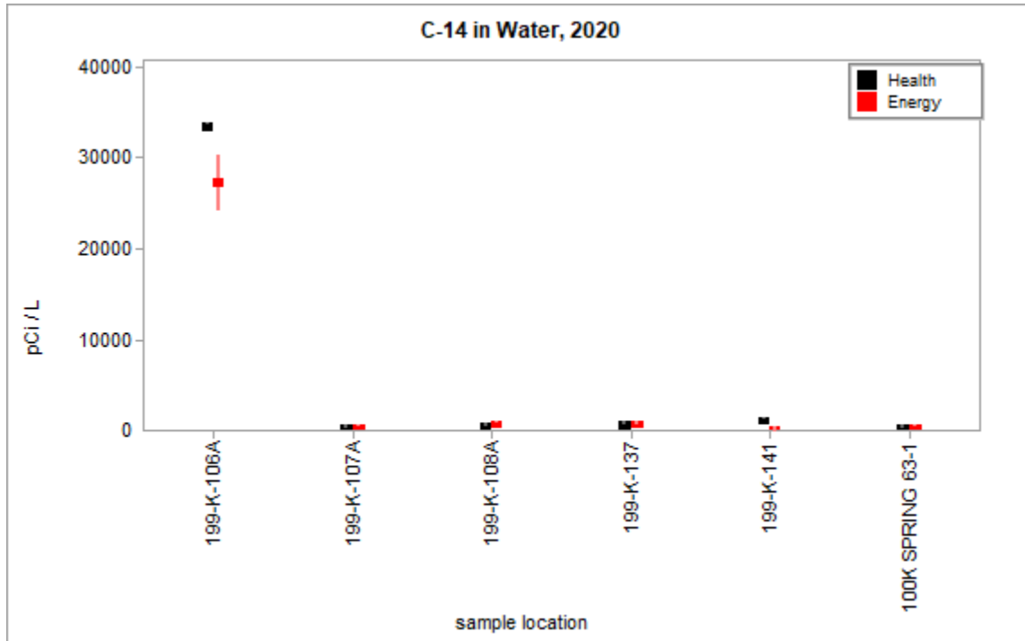
Figure 3.2.2 – Health and Energy C-14 Concentrations in Water, All Data
