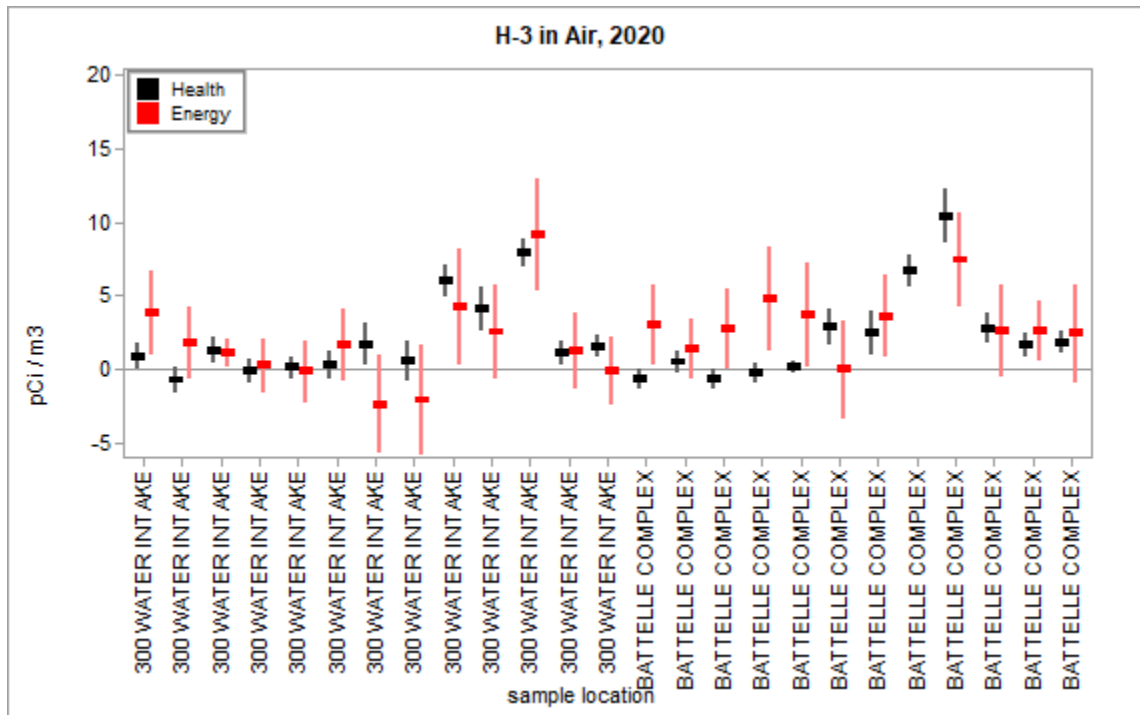
Figure 3.1.7 – Health and Energy H-3 Concentrations in Air
