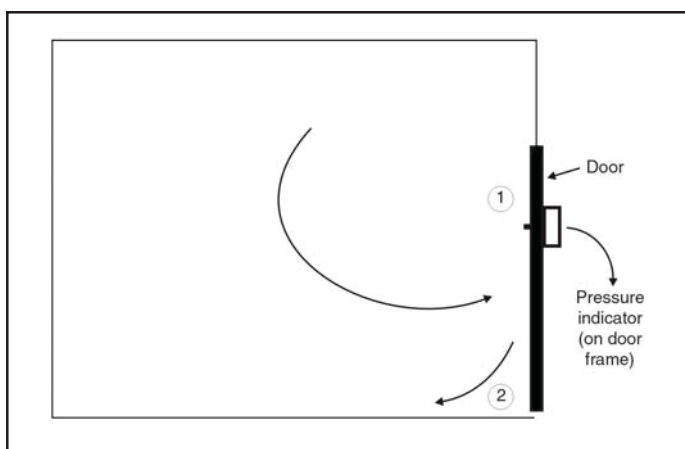
FIGURE 6. Cross-sectional view of a room indicating the location of negative pressure measurement*
