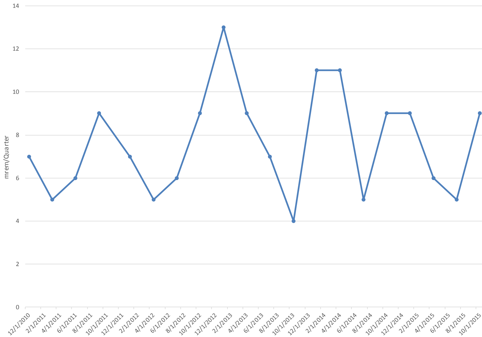
Dose mrem/Quarter Corrected Location 14
