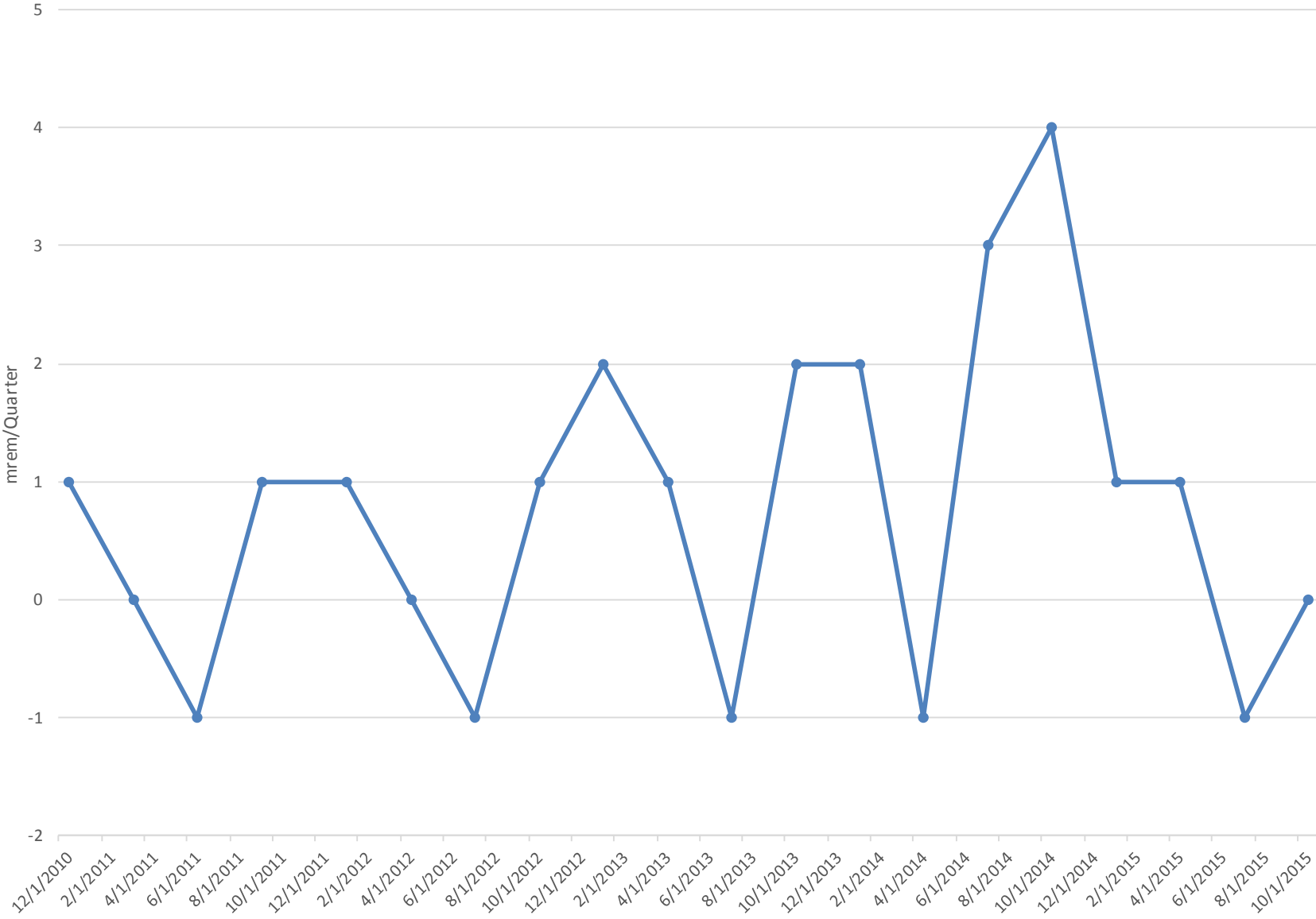
Dose mrem/Quarter Corrected Location 15
