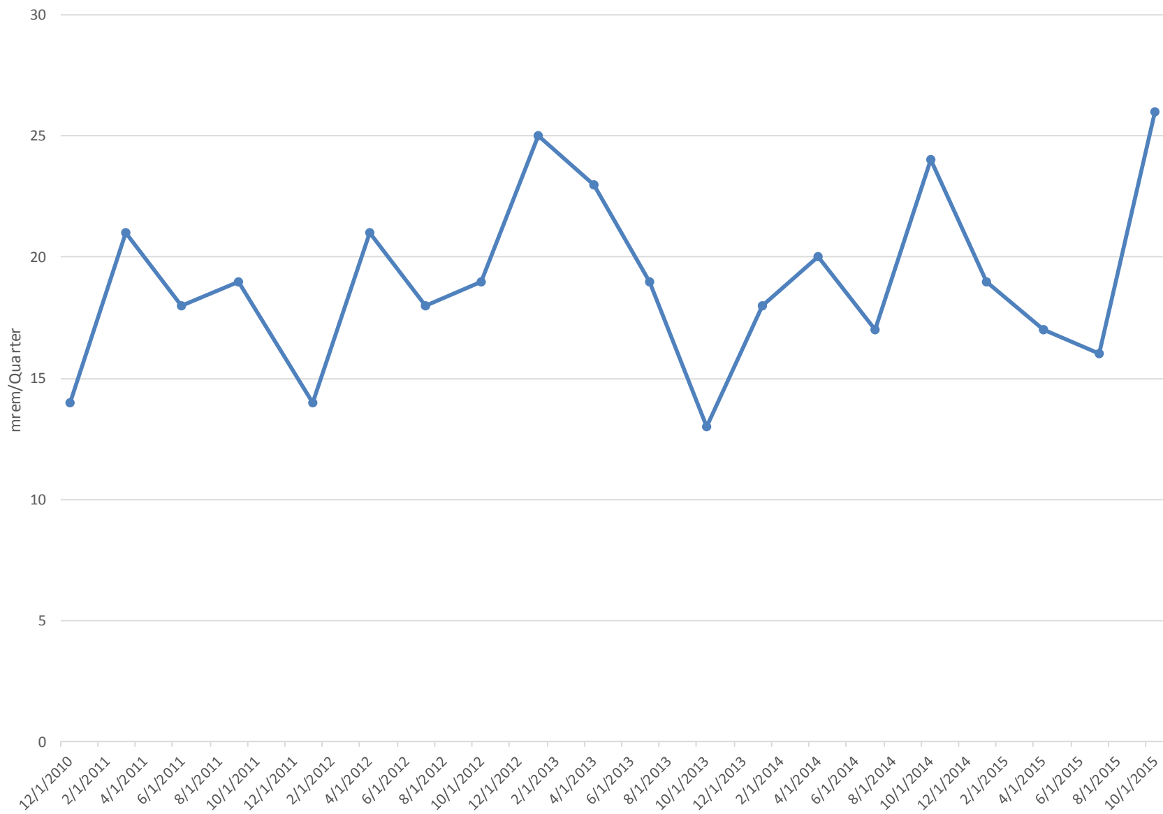
Dose mrem/Quarter Corrected Location 11
