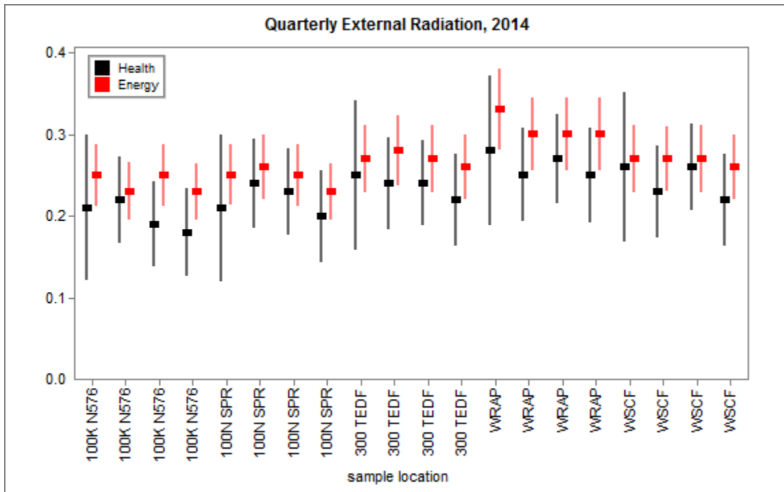
Figure 3.3.2 Health and Energy Quarterly External Radiation
