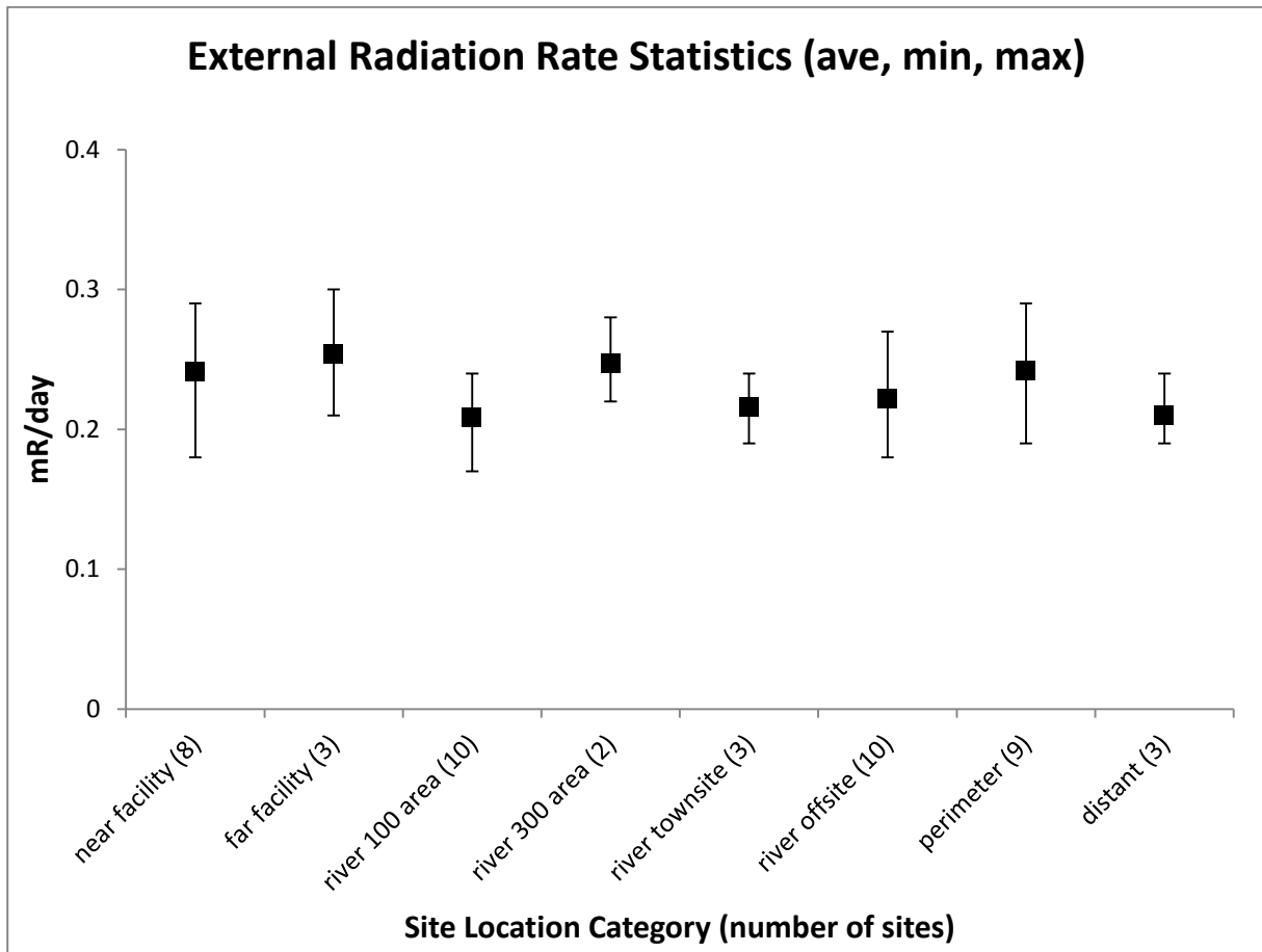
Figure 3.3.4 External Radiation Rate Statistics by Location Type
