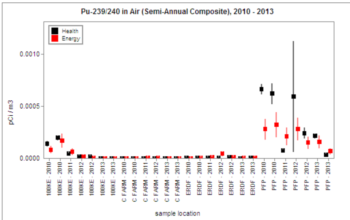
Figure 3.1.19 Health and Energy Pu-239/240 Concentrations in Air
