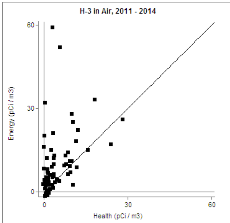
Figure 3.1.10 Health and Energy Scatter Plot for H-3 Concentrations in Air
