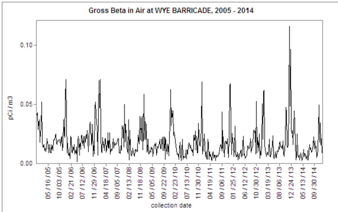
Figure 3.1.22 Health’s Historical Gross Beta Concentrations in Air at Wye Barricade
