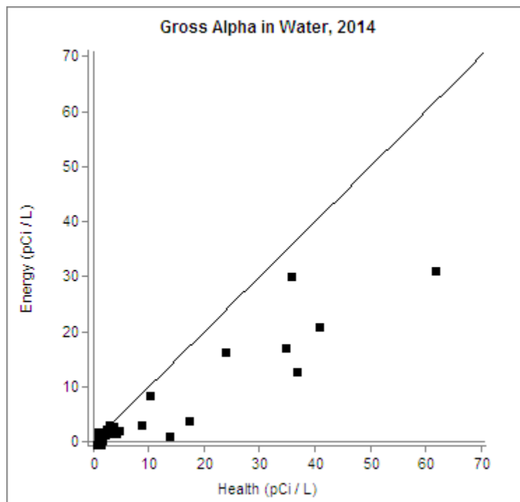
Figure 3.2.5 Health and Energy Scatter Plot for Gross Alpha Concentrations in Water
