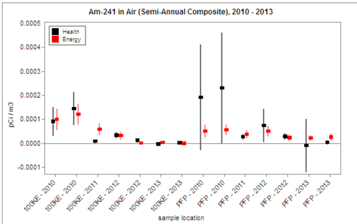
Figure 3.1.11 Health and Energy Am-241 Concentrations in Air, 2010 - 2013
