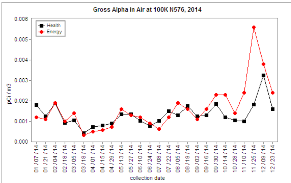
Figure 3.1.3 Health and Energy Gross Alpha Concentrations in Air at 100K N576
