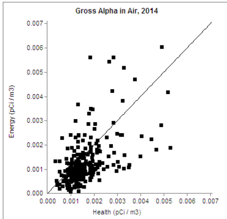
Figure 3.1.4 Health and Energy Scatter Plot for Gross Alpha Concentrations in Air
