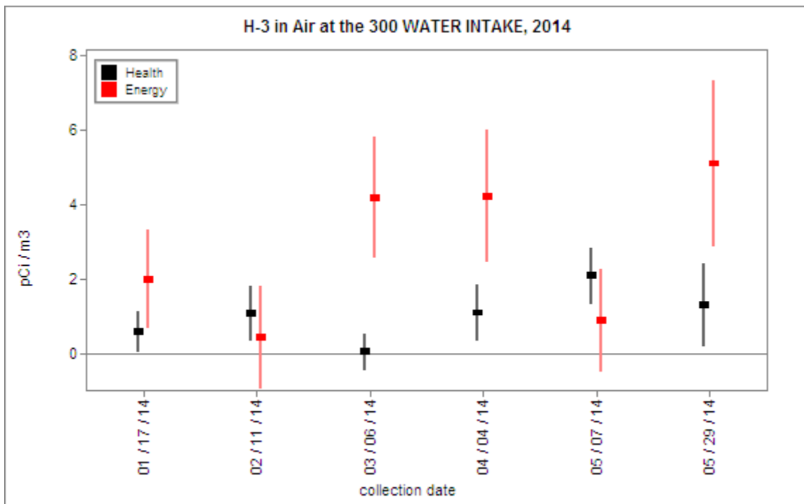
Figure 3.1.9 Health and Energy H-3 Concentrations in Air at the 300 Water Intake
