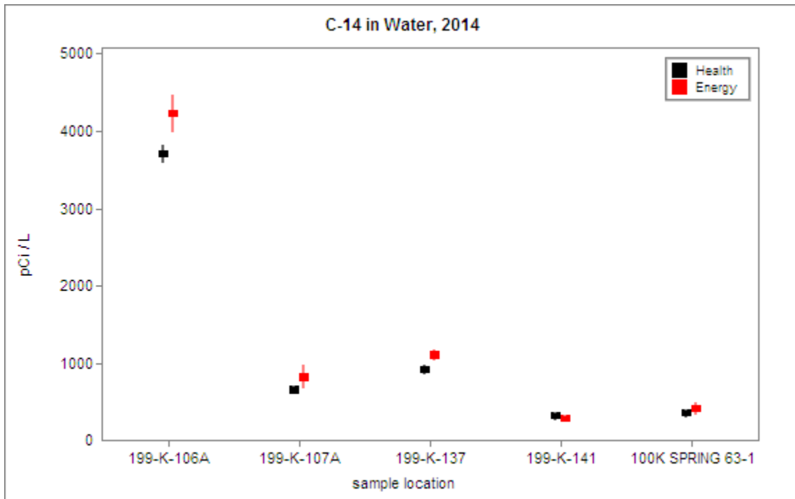
Figure 3.2.2 Health and Energy C-14 Concentrations in Water Samples
