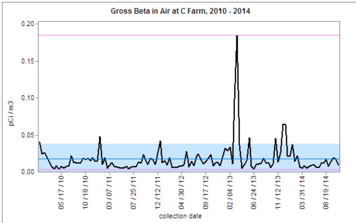
Figure 3.1.8 Health's Gross Beta Concentrations in Air at C Farm
