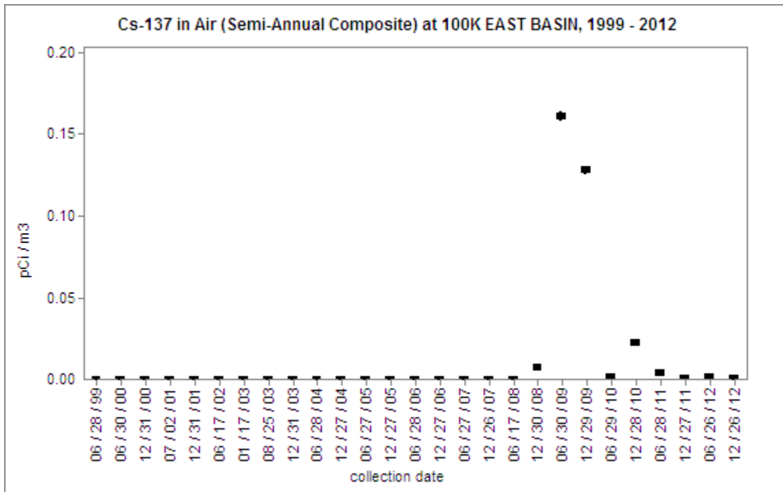
Figure 3.1.14 Health's Historical Cs-137 Concentrations in Air at 100K East Basin
