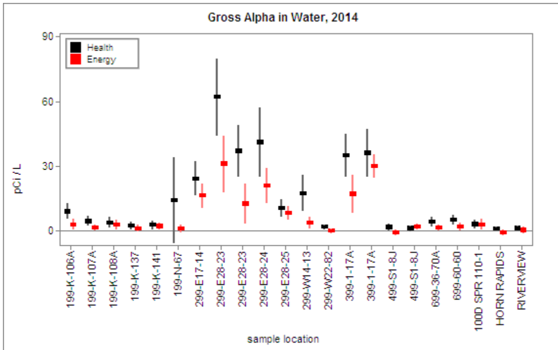
Figure 3.2.4 Health and Energy Gross Alpha Concentrations in Water Samples
