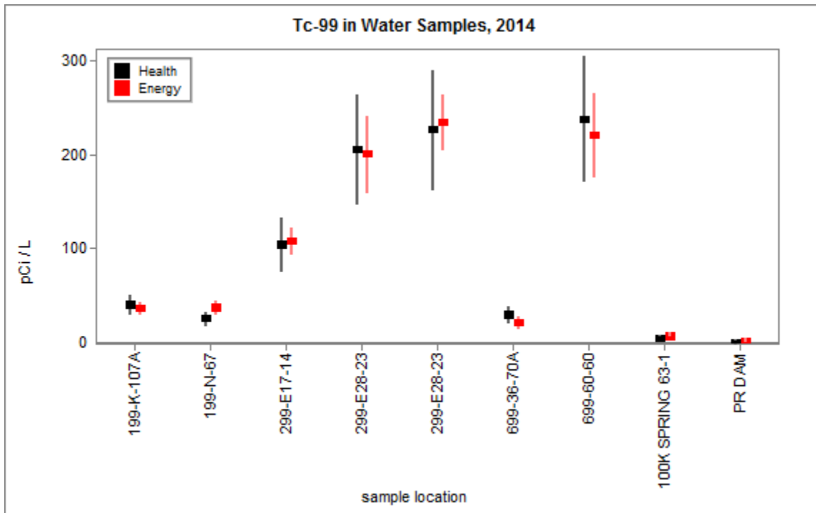
Figure 3.2.6 Health and Energy Tc-99 Concentrations in Water Samples
