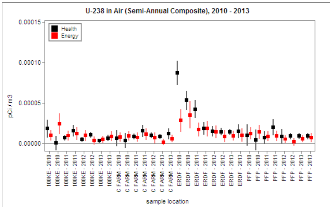
Figure 3.1.21 Health and Energy U-238 Concentrations in Air
