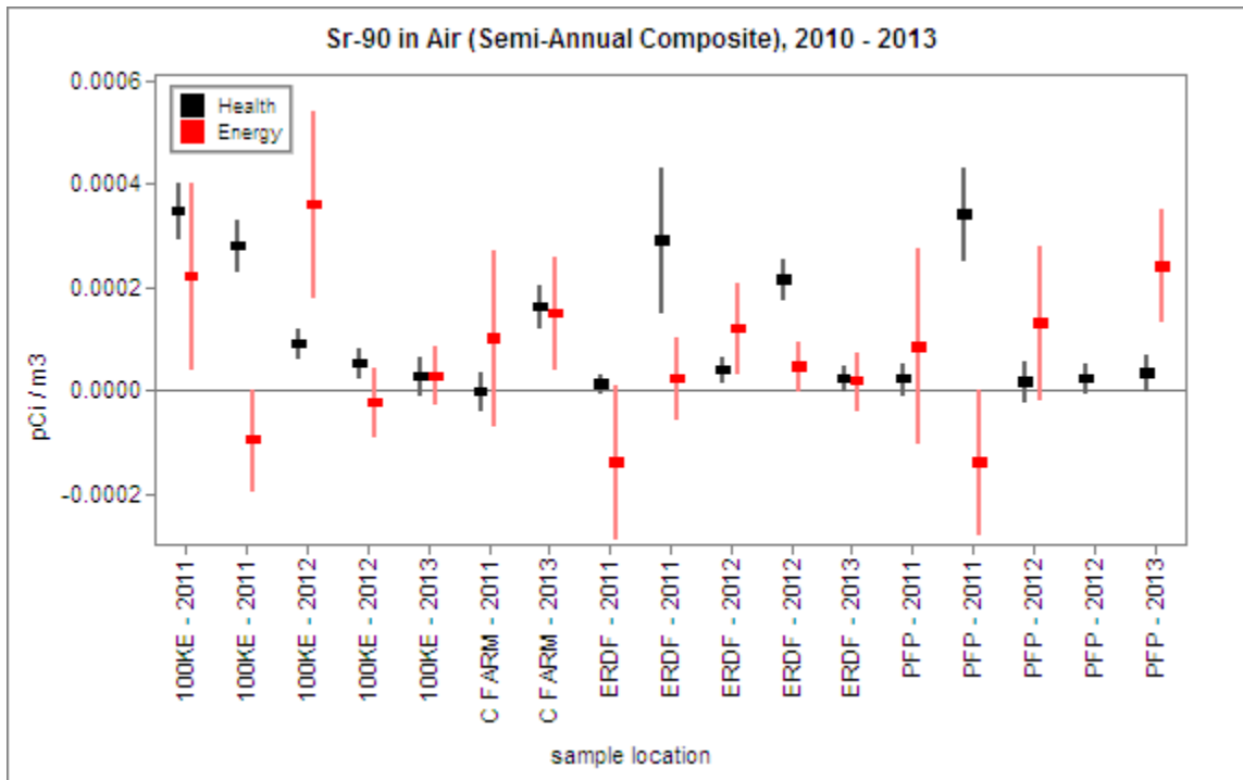
Figure 3.1.20 Health and Energy Sr-90 Concentrations in Air
