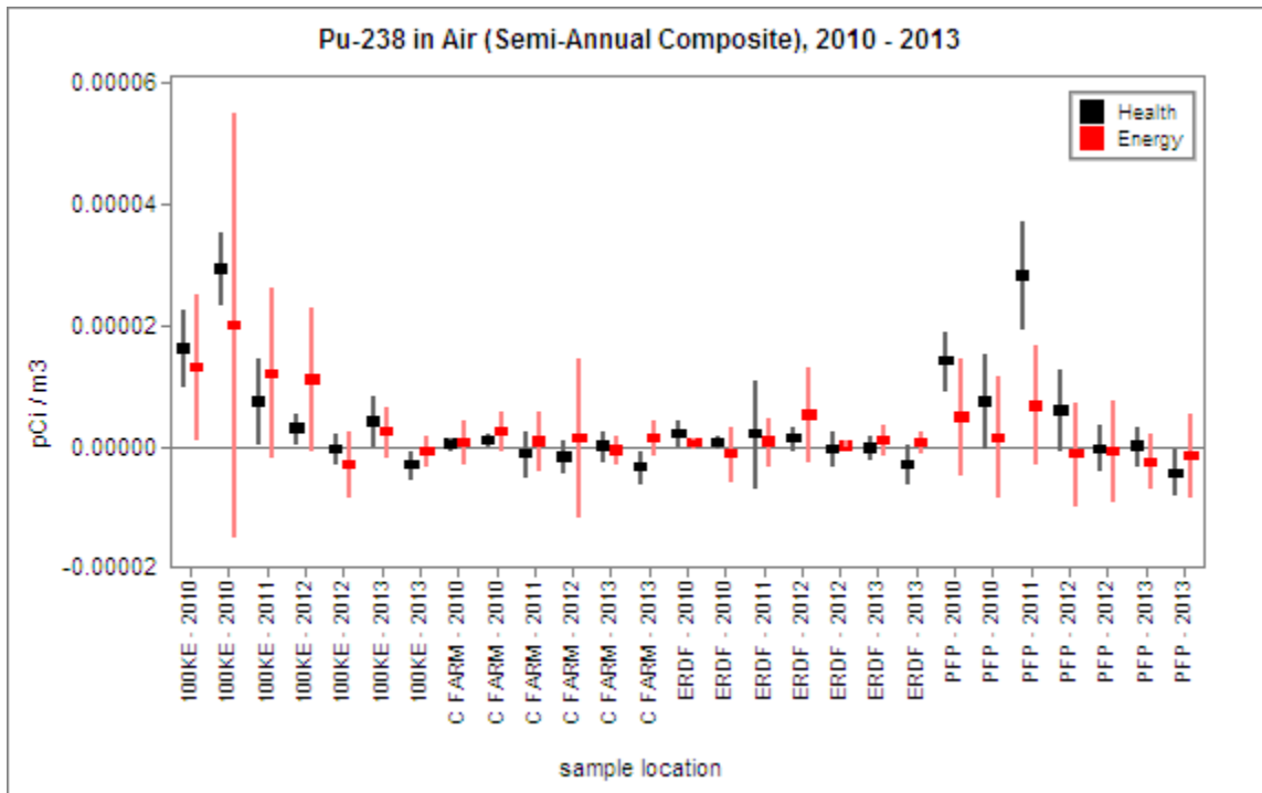
Figure 3.1.18 Health and Energy Pu-238 Concentrations in Air
