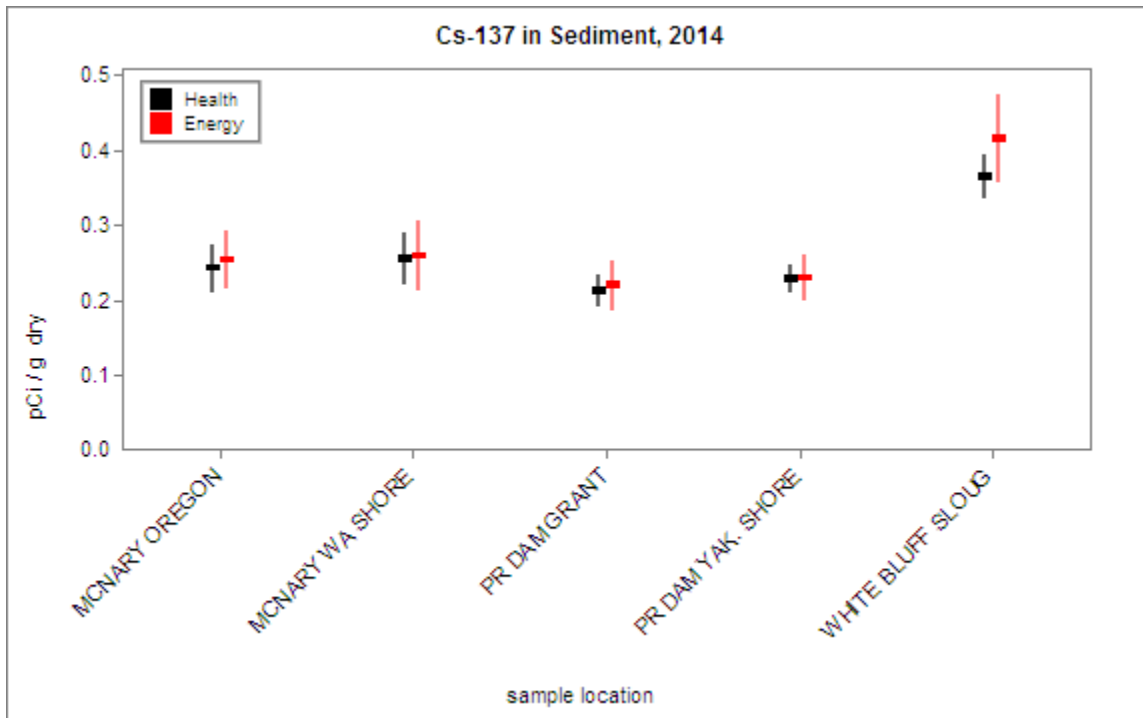
Figure 3.4.2 Health and Energy Cs-137 Concentrations in Sediment
