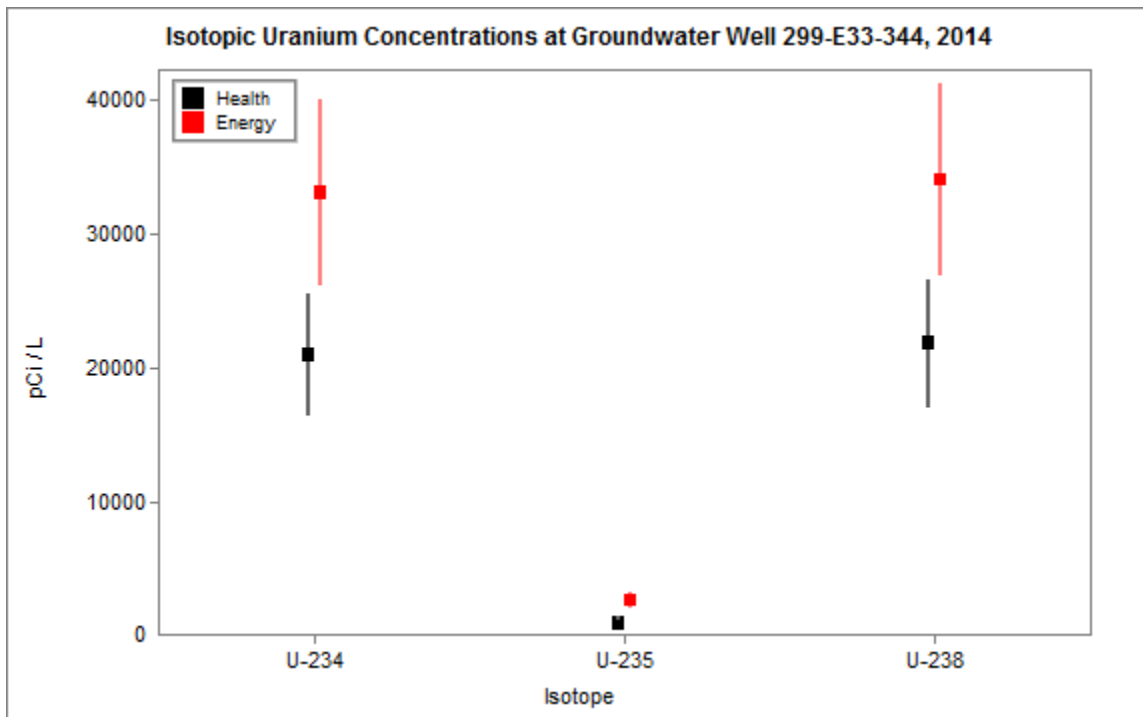
Figure 3.2.7 Health and Energy Isotopic Uranium Concentrations at 299-E33-344
